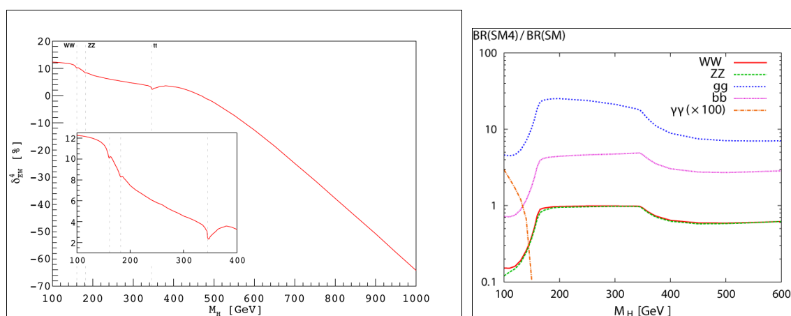
Figure 1: (left) NLO EW correction to the ggF Higgs production in SM4. (right) Ratio of BR in SM4/SM calculated with Prophecy4f and HDECAY .
