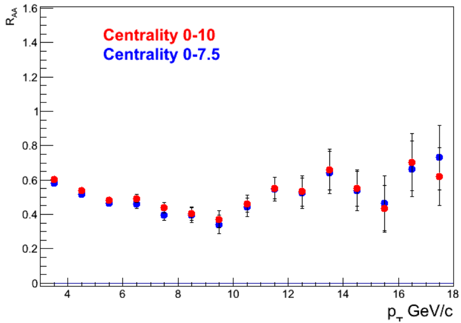
Heavy flavor electron RAA
