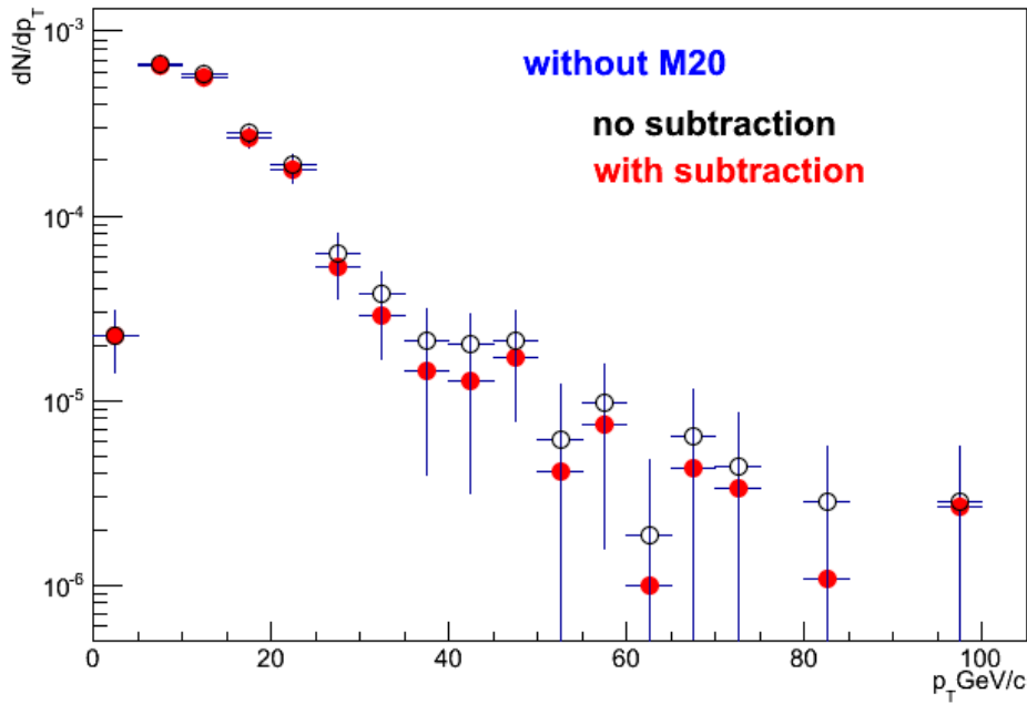
jet tagged by HFE
