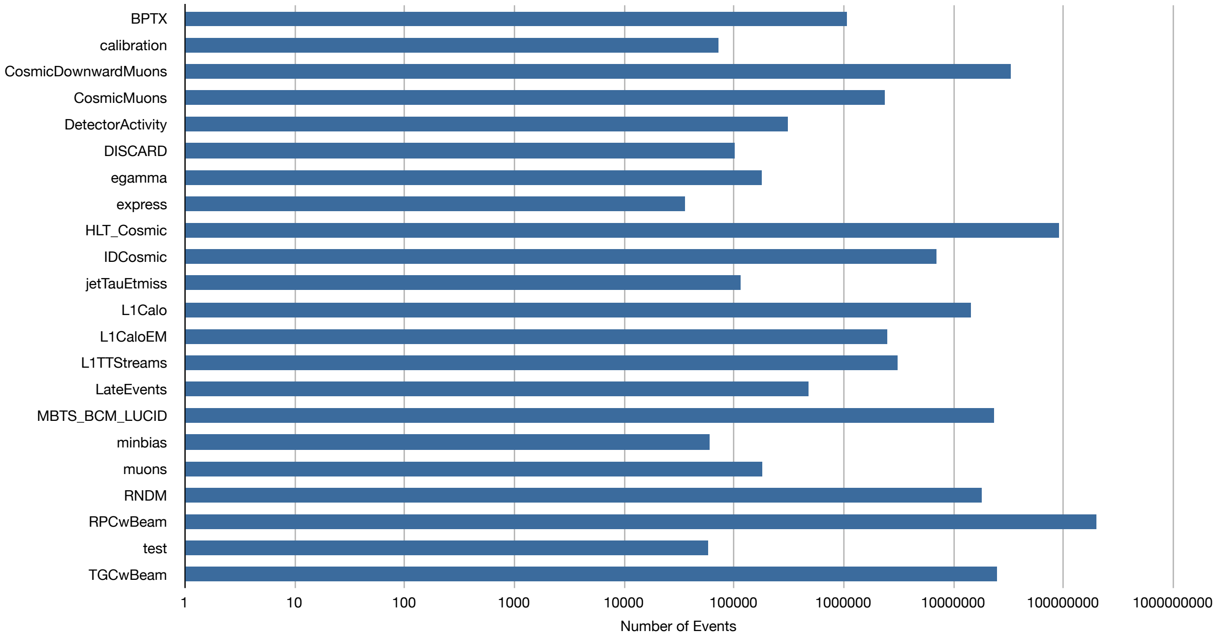
Physics stream event distribution for Cosmic data from August 1 to October 31, 2008
