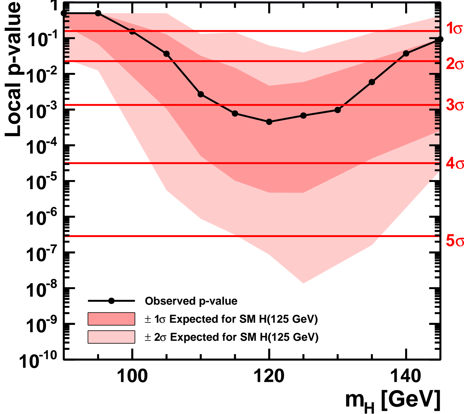
CMS (unpublished) H \rightarrow \tau\tau , 4.9 \text{ fb}^{-1} at 7 TeV, 19.7 \text{ fb}^{-1} at 8 TeV
