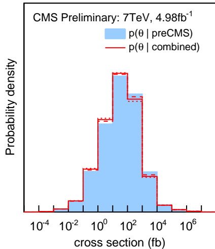
p(\theta | \text{EWKino})
