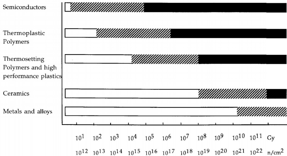
Figure 1: General appreciation of radiation damage to materials (from [6]). No damage (blank), mild to severe (shaded) or destruction (black). The horizontal axis shows the ionizing dose in Gy and the approximate equivalent neutron fluence (note that the effect of 1 Gy roughly corresponds to 10 11 neq/cm 2 ).
