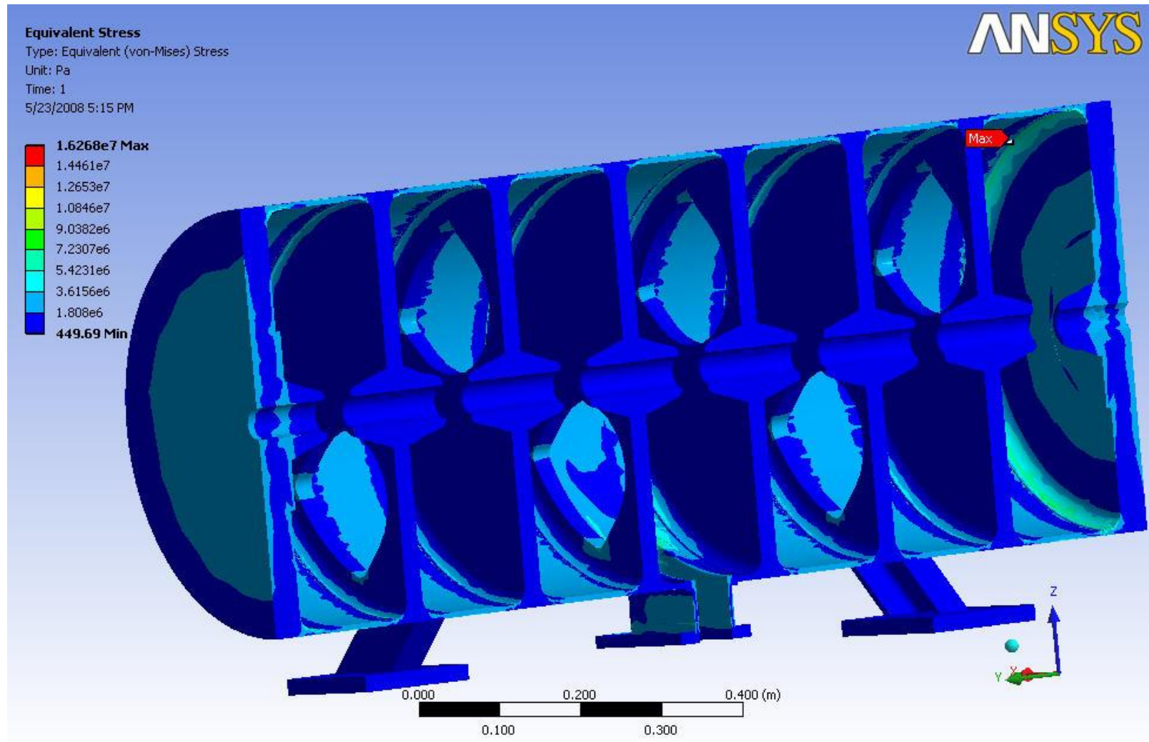
PIMS STRESS PM THE COUPLING SLOTS
