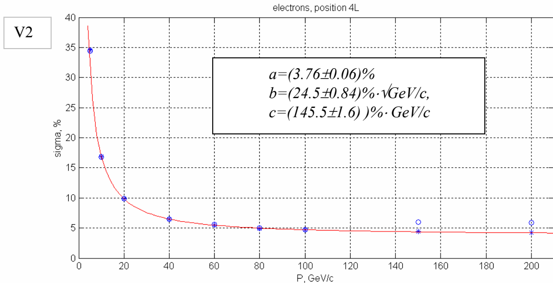
Figure 3: FCAL1 energy resolution for electrons in position 4L, with r_{core}=8\text{cm} , for the definition V2 of norm_m . The points are: \circ – calibration off, * – calibration on. The line shows the fit with the function \sigma = a \oplus \frac{b}{\sqrt{P}} \oplus \frac{c}{P} (P in GeV/c). With the alternative definition V1, the data points and the fit are indistinguishable from V2.
