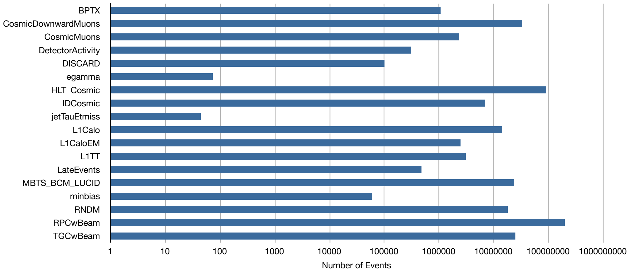
Physics stream event distribution for Cosmic data from August 1 to October 31, 2008
