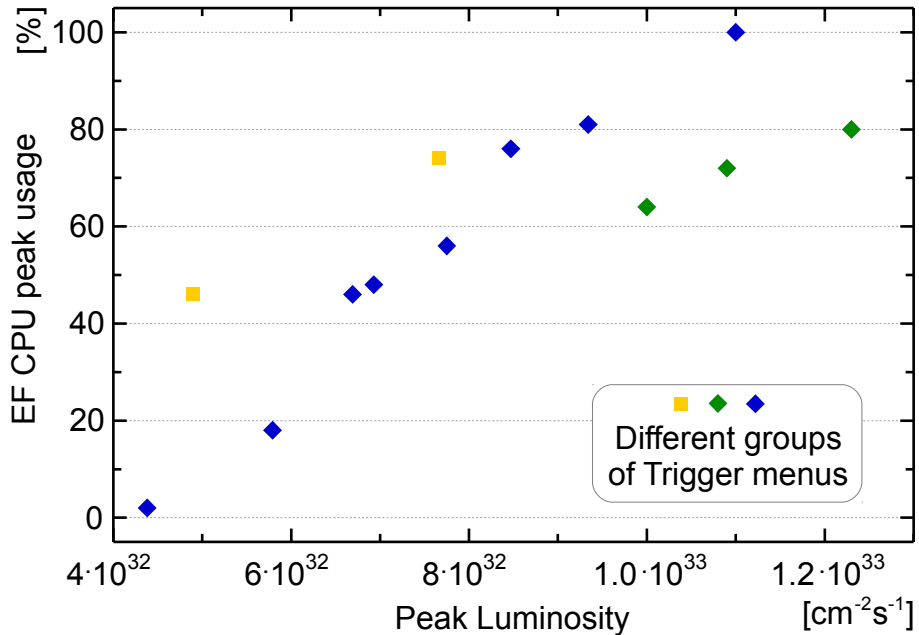
EF CPU usage vs. Luminosity
