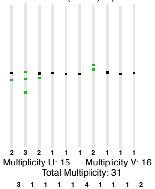
Station 2 (B7L1L) U plane
