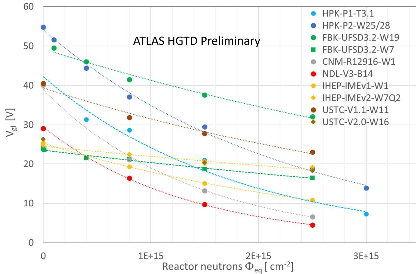
Gain layer depletion voltage dependence on equivalent fluence of reactor neutrons for different investigated prototype sensors ( producer-run-wafer ). The dashed lines are the acceptor removal model (exponential) fits to the data.
