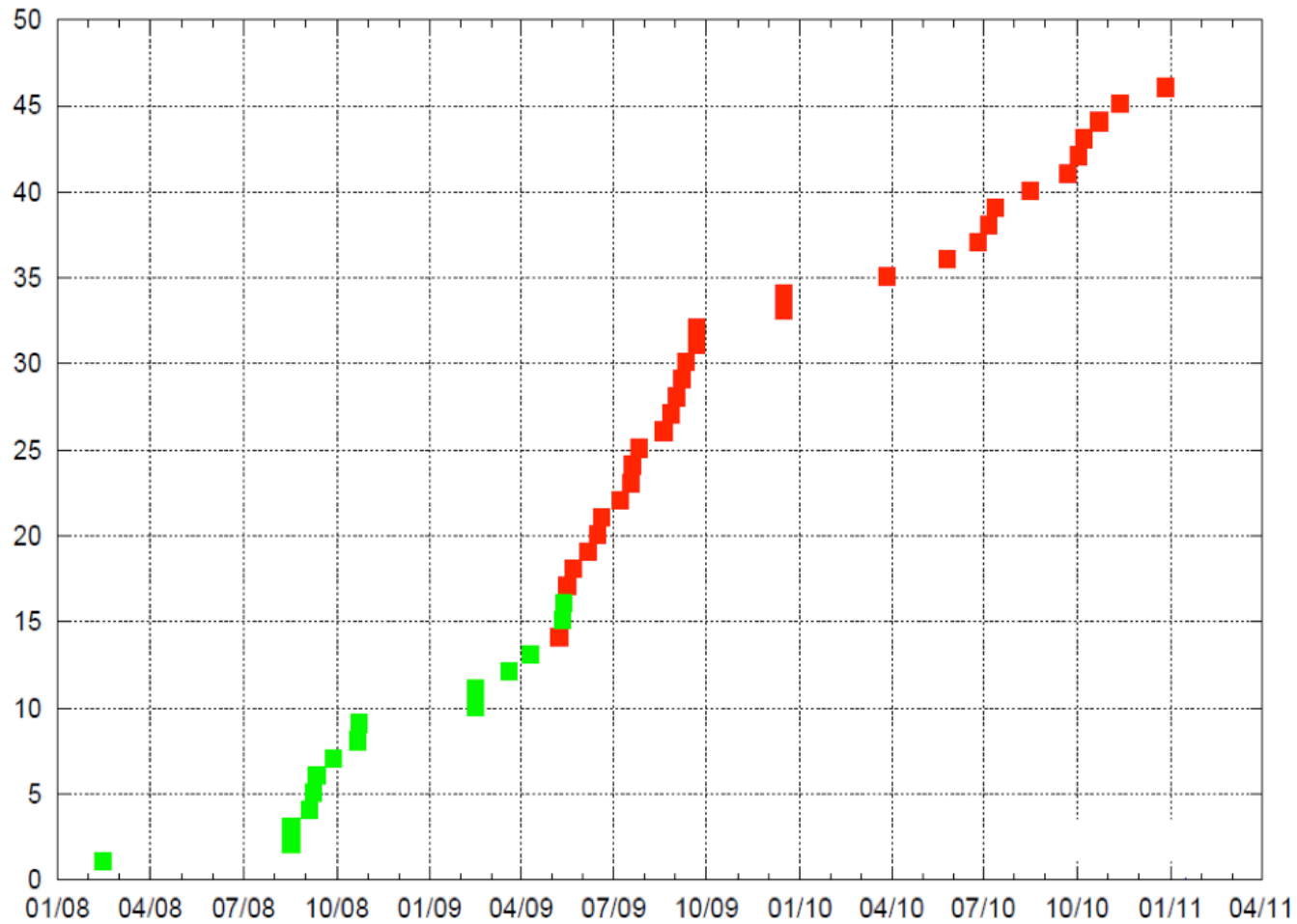
Distribution of the cumulative Optical Transmitter (OTx) failures between as a function of time since January 2008. The green markers indicate front-end boards (FEB) replaced during the shutdown in the beginning of 2009 and the red markers indicate the failures since.
