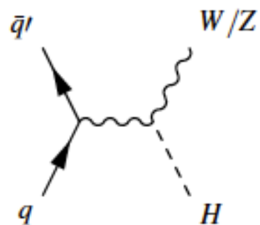
(c) VH
