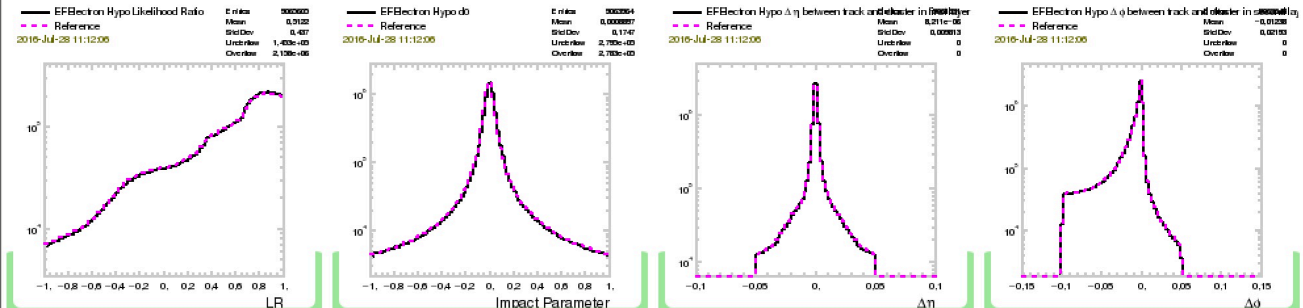
EFElectronHypo_e24_lhmedium_LikelihoodR, TrgEFElectronHypo_e24_lhmedium_d0, TrgEFElectronHypo_e24_lhmedium_dEta, TrgEFElectronHypo_e24_lhmedium_dPhi
