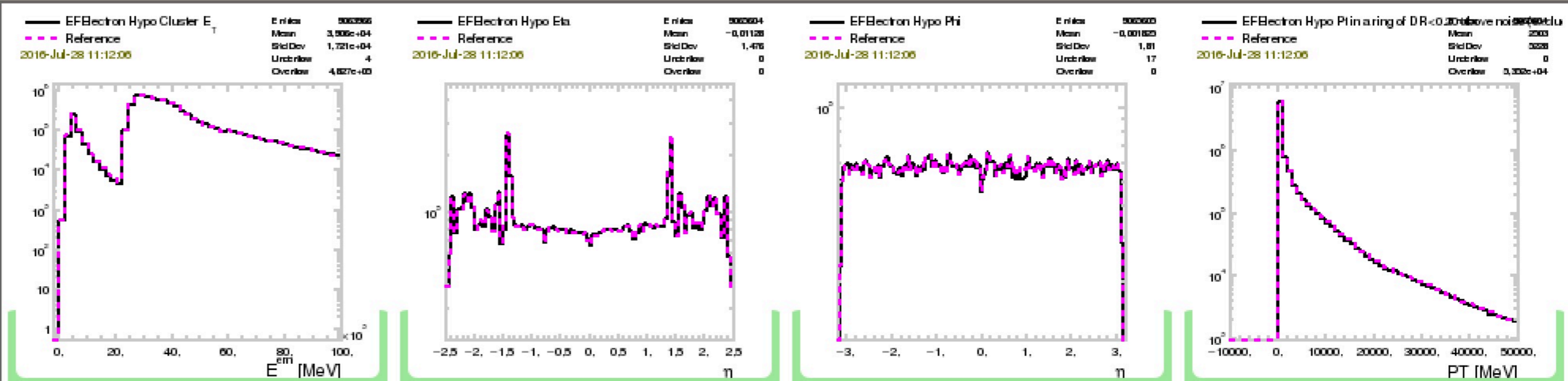
TrgEFElectronHypo_e24_lhmedium_El_Cluster, TrgEFElectronHypo_e24_lhmedium_El_Eta, TrgEFElectronHypo_e24_lhmedium_El_Phi, TrgEFElectronHypo_e24_lhmedium_El_PtCone
