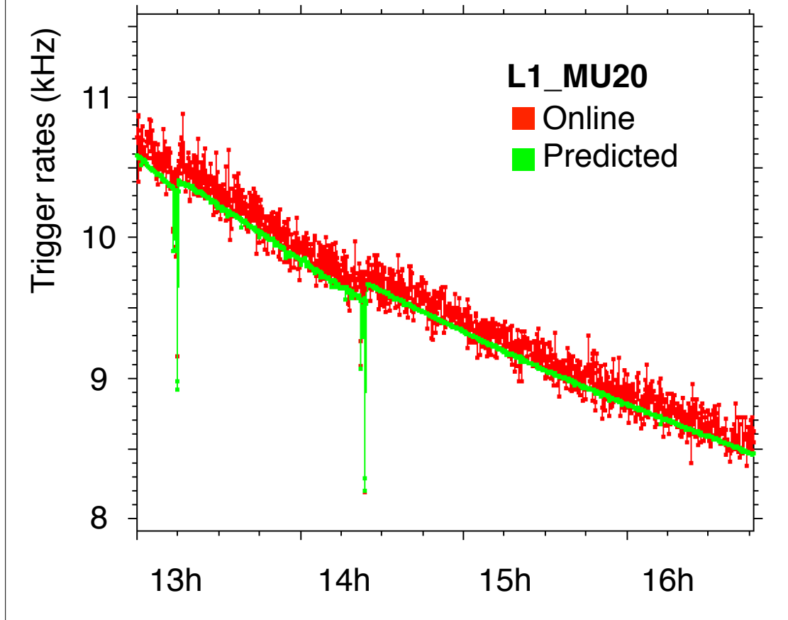
Caption: Level-1 trigger rates online (red) compared with predictions based on luminosity-scaling (green) for the algorithm noted in the plot. The downward spikes correspond to the luminosity optimization done by the LHC.
