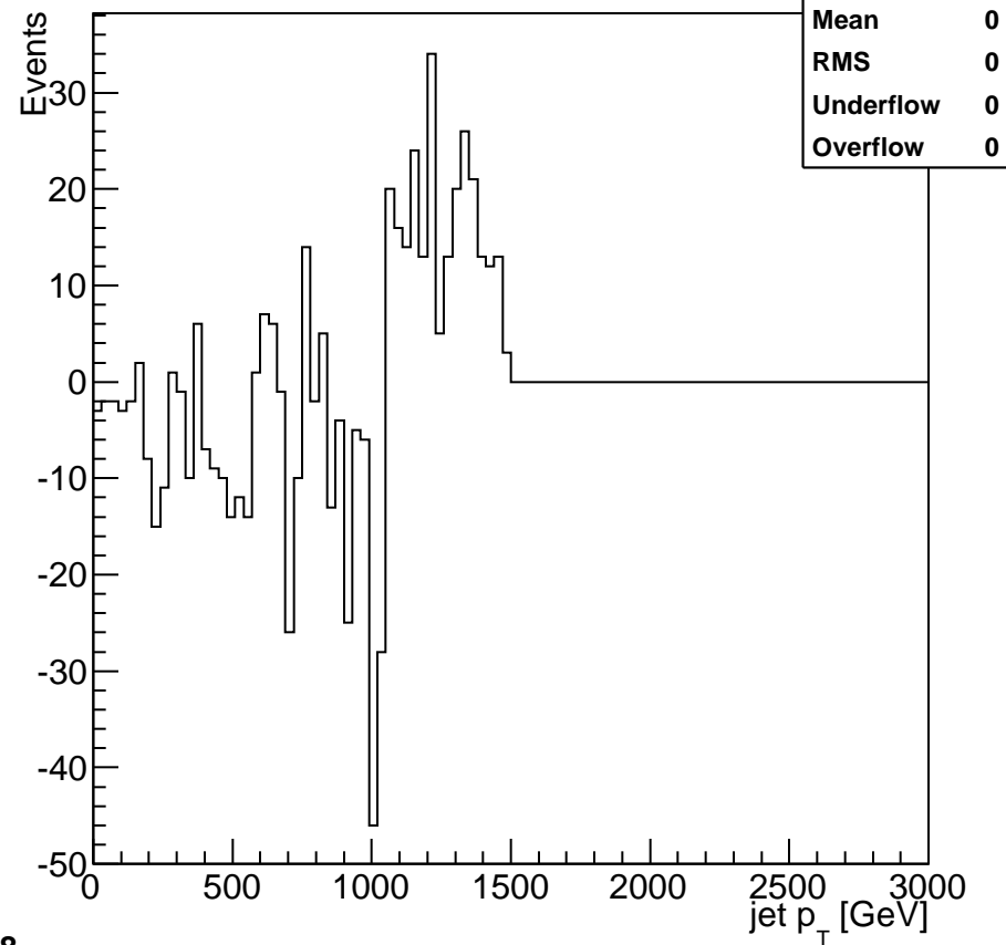
Leading jet p T (diff)
