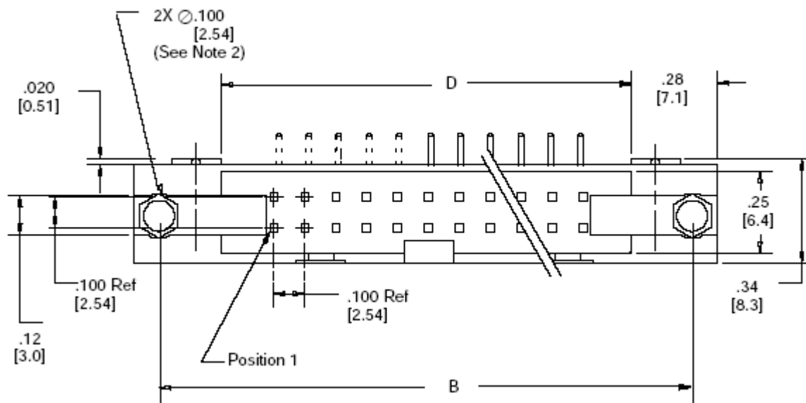
Figure 2: Connector layout with the position of pin 1 for the connector 3M 3431-5502.
