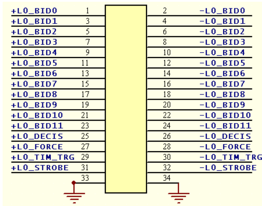
Figure 1 : L0 trigger input on the Readout Supervisor. The pair called L0_STROBE is not used anymore but is instead a spare connection.
