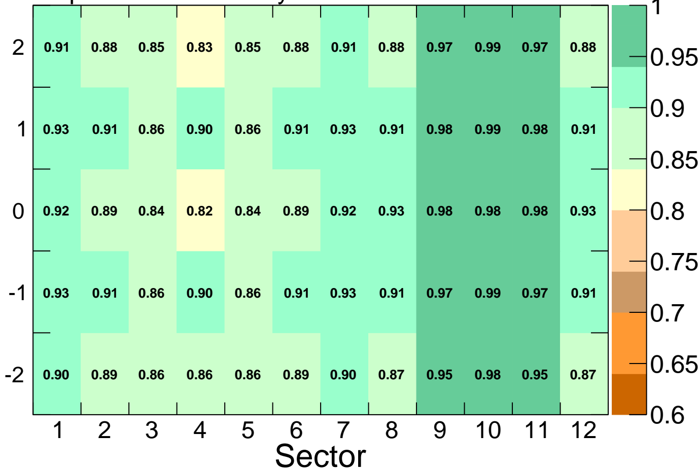
Expected hit efficiency of the MB4 chambers
