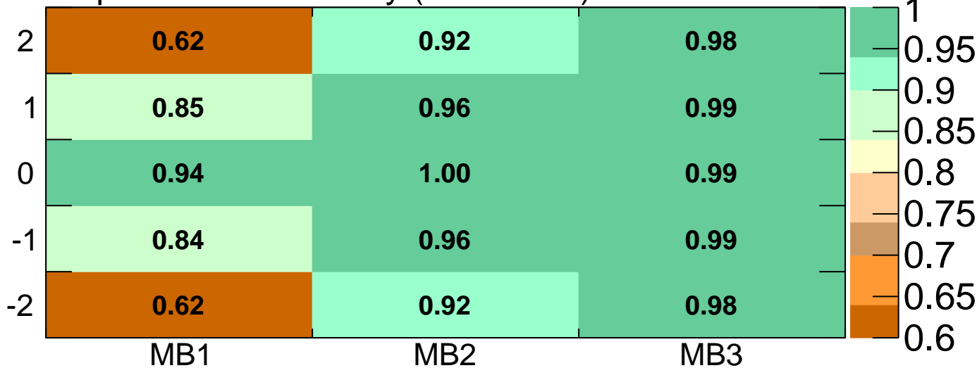
Expected hit efficiency (all sectors)
