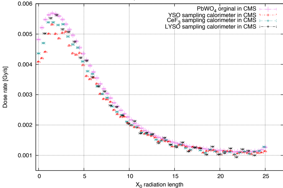
Dose rate, samp calo vs. \text{PbWO}_4 original, 8 \cdot 10^9 pp int./s, 1.8 < \eta < 2.6
