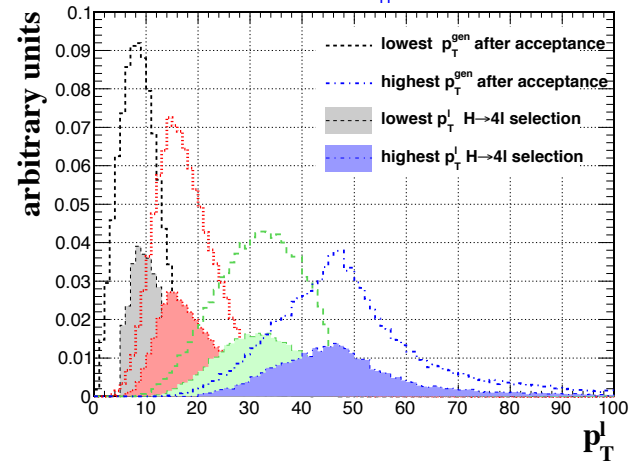
H \rightarrow ZZ^* \rightarrow 2e2\mu , m_H = 140 GeV
