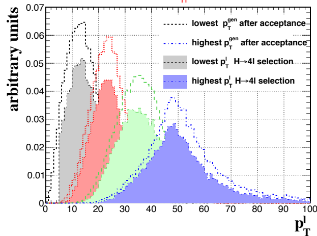
H \rightarrow ZZ^* \rightarrow 4\mu , m_H = 140 GeV
