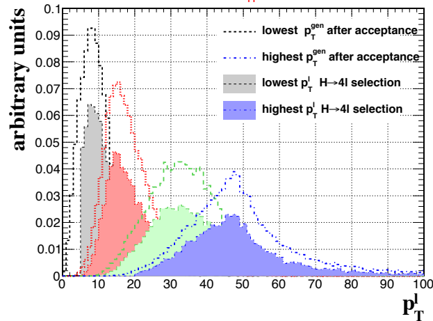
H \rightarrow ZZ^* \rightarrow 4\mu , m_H = 140 GeV
