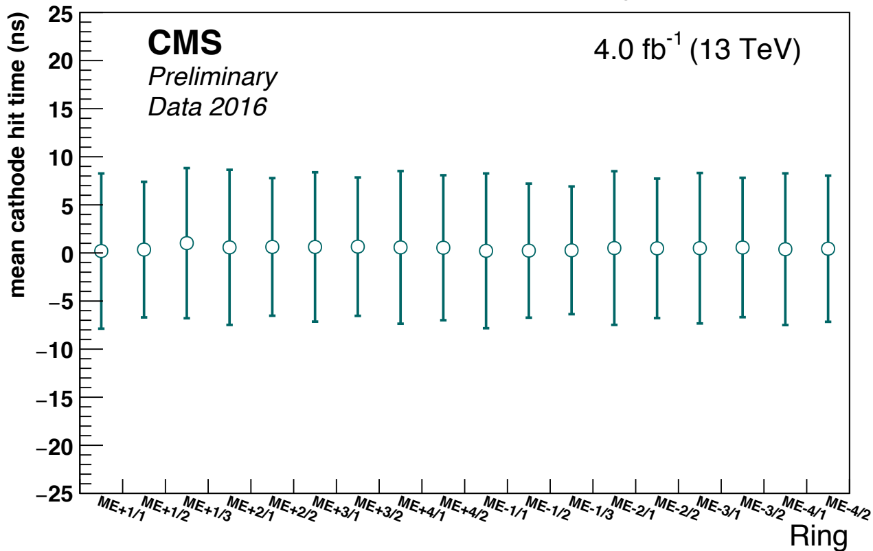
Mean and RMS of cathode hit time for each ring of CSC chambers
