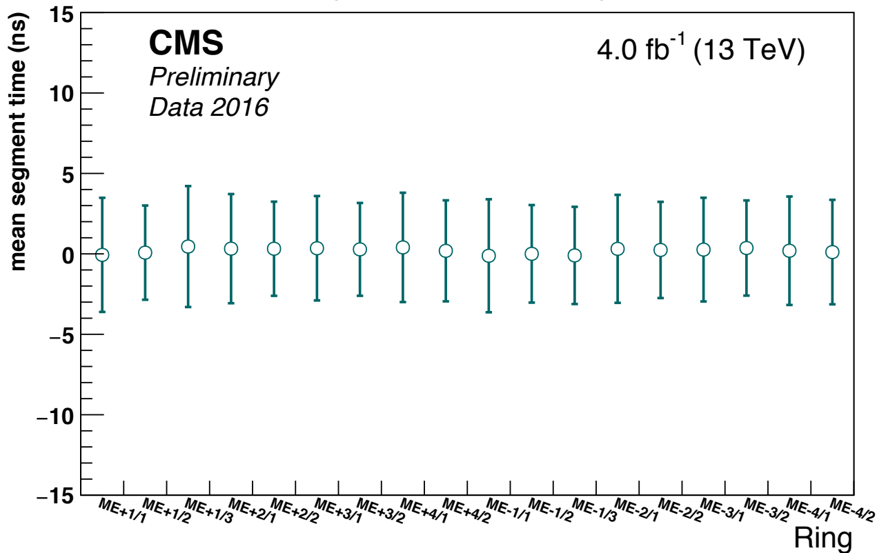
Mean and RMS of segment time for each ring of CSC chambers
