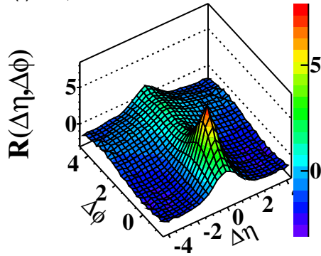
(c) CMS \sqrt{s} = 7\text{TeV}
