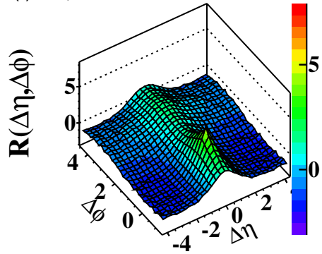
(a) CMS \sqrt{s} = 0.9\text{TeV}
