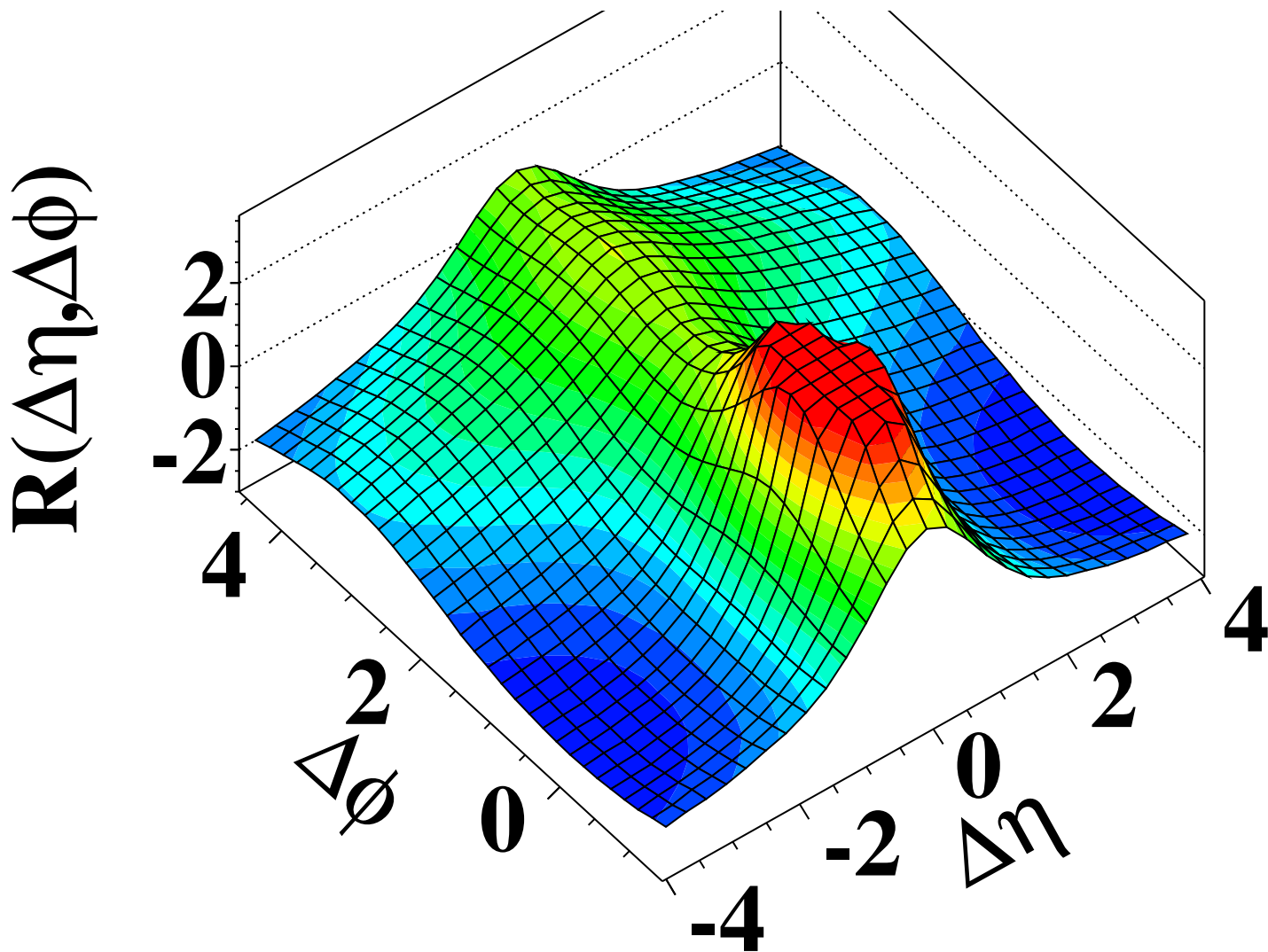
(a) CMS MinBias, p_T > 0.1 \text{ GeV}/c
