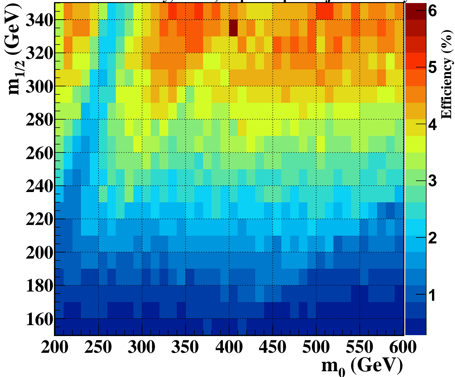
CMS Preliminary, 7 TeV, 36 pb -1 . Lepton + jets efficiency
