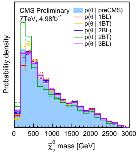
p(\theta | \text{HT} + \text{MET} + \text{b-jets})
