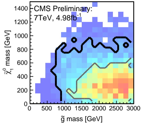
p(\theta | \text{HT + MHT combined})
