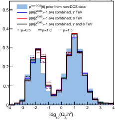
pMSSM, CMS preliminary
