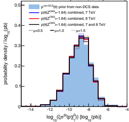
pMSSM, CMS preliminary
