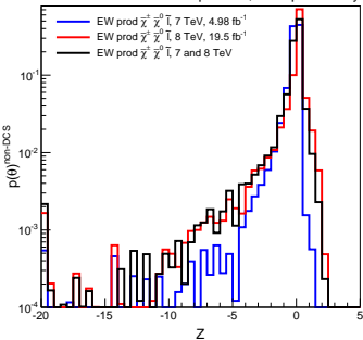
pMSSM, CMS preliminary
