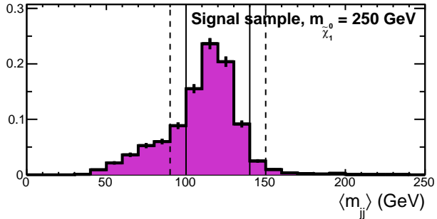
CMS Simulation, L = 19.3 \text{ fb}^{-1} , \sqrt{s} = 8 \text{ TeV}
