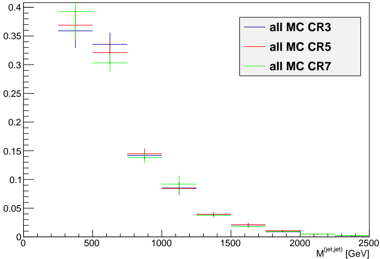
M_{jj} distribution for different \tau isolation regions
