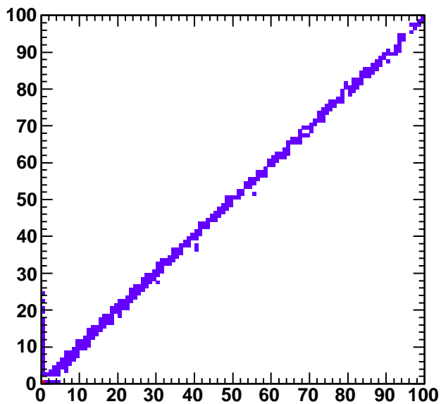
HB RecoHit_E vs TP_E
