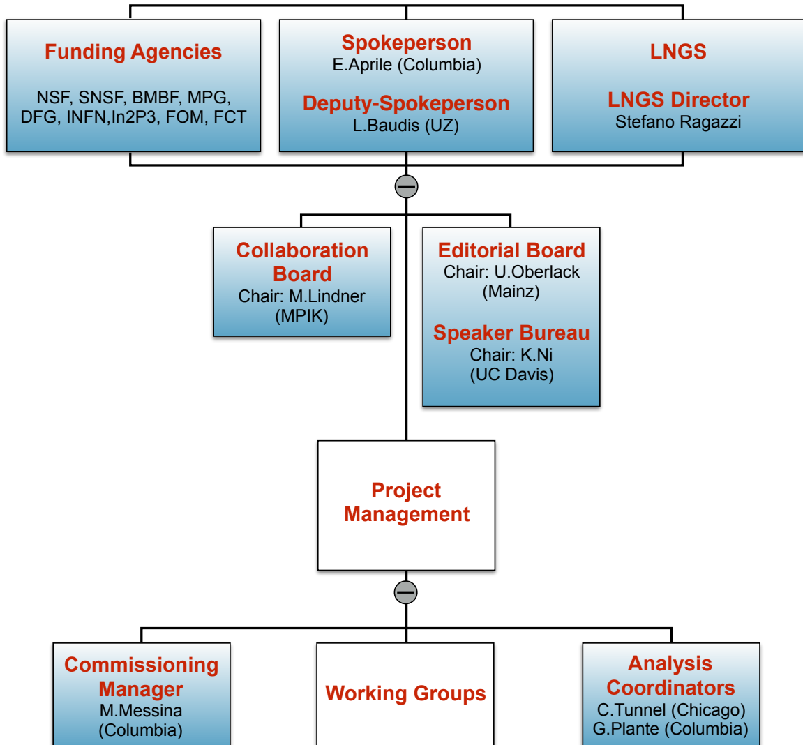
FIGURE 1: ORGANIZATION OF THE XENON1T COLLABORATION.
