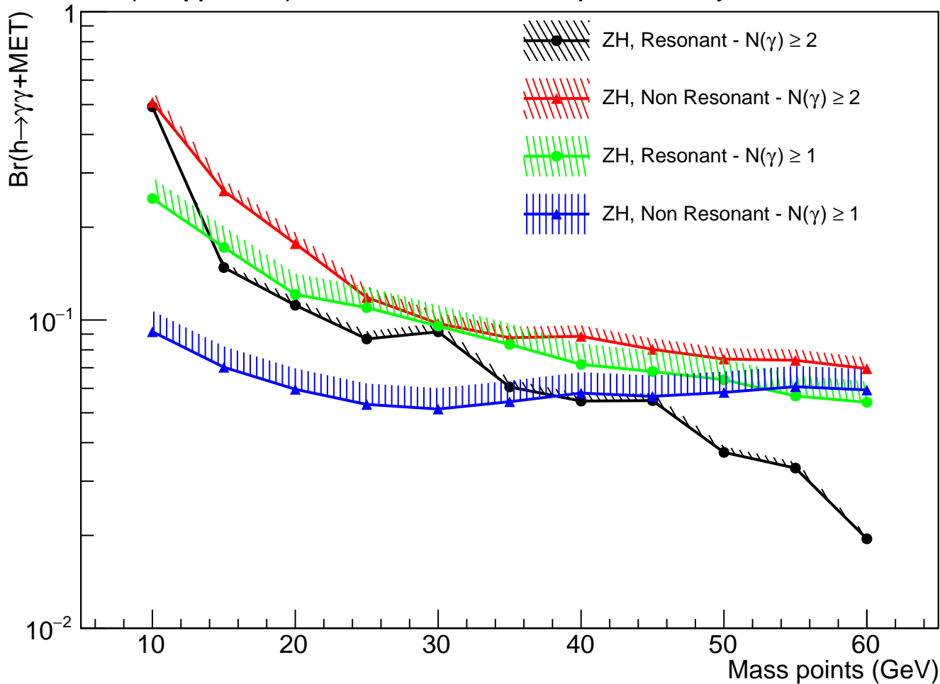
Br( h \rightarrow \gamma\gamma + \text{MET} ) for 95% CL exclusion plus 10% systematic band
