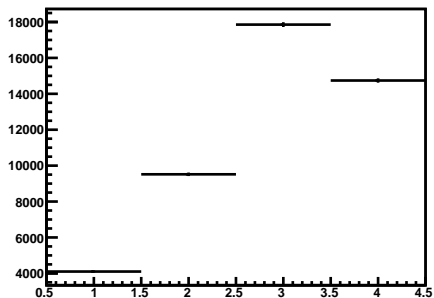
MS X position at M2 for IML tracks
