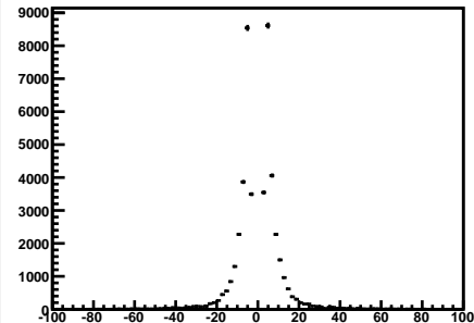
IsMuonLoose Candidate Momentum (GeV/c^2)
