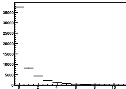
MS Y position at M2 for IML tracks
