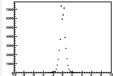
IsMuonLoose Candidate p_T (GeV/c^2)
