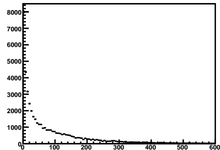
IsMuon Dist for IML candidates
