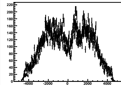
MS X position at M2 for IML tracks
