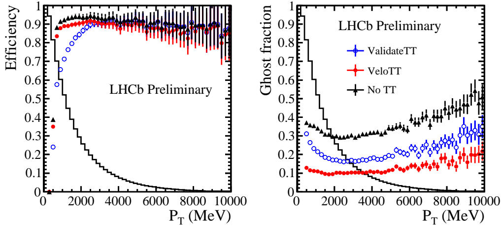
Figure 2: Tracking performances for three options in the usage of the TT-stations in the pattern recognition sequence, evaluated on Monte Carlo simulated events at 13 TeV: TT-stations not considered for the pattern recognition (NoTT, triangles); validation of VELO seeds with TT-stations (ValidateTT, open circles); momentum estimate with the TT-stations (VeloTT, full circles). Left: efficiency as a function of the generated particle p_T . Right: ghost rate as a function of the generated particle p_T . The background histograms displays the generated p_T distribution. Electrons are excluded from the study.
