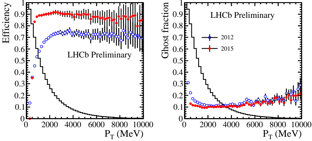
Figure 1: Comparison of the 2012 tracking sequence (no IP selection applied, open circles) with the 2015 tracking sequence (full circles), evaluated on Monte Carlo simulated events at 13 TeV. Left: efficiency as a function of the generated particle p_T . Right: ghost rate as a function of the generated p_T . The background histograms displays the generated p_T distribution. Electrons are excluded from the study.
