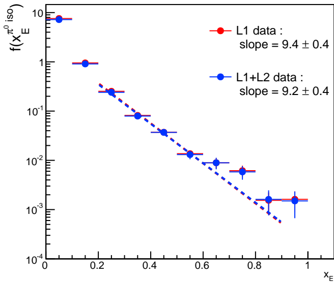
Total x_E distribution for isolated \pi^0 with purity scaling
