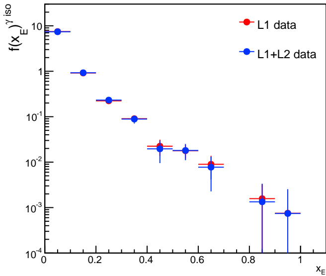
x_E distribution for isolated photons
