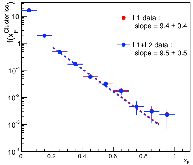
x_E distribution for isolated clusters scaling with purity
