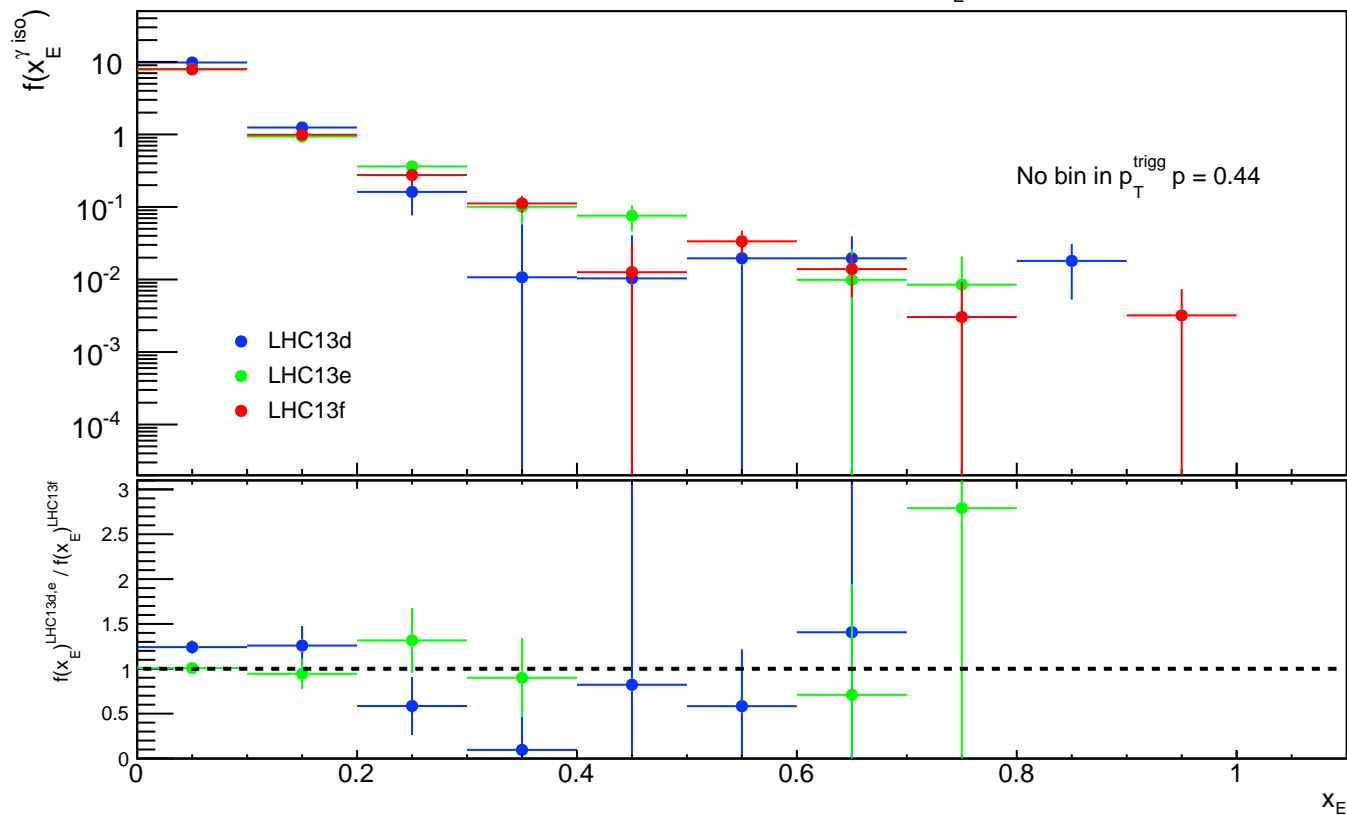
Ratio between LHC13d, LHC13e and LHC13f x_E distribution
