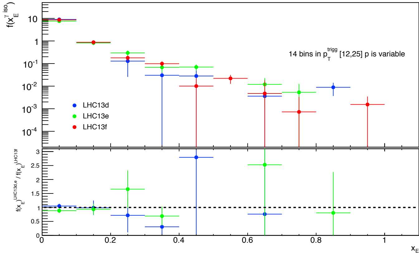
Ratio between LHC13d, LH13e and LHC13f x_E distribution
