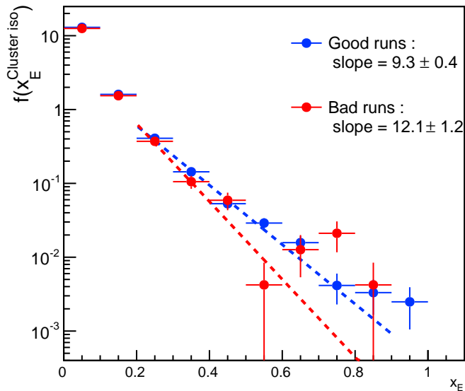
x_E distribution for isolated clusters
