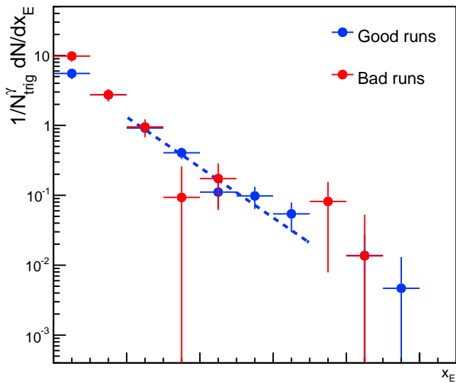
x_E distribution for isolated \pi^0
