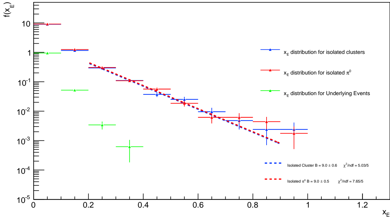
x_E distribution for isolated clusters, isolated \pi^0 and Underlying Events
