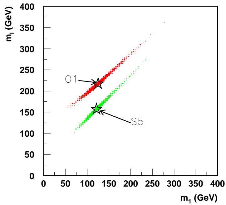
Figure 15: Reconstructed m_f versus m_{\tilde{\chi}_1^0} for O1 and S5 . The stars show the true masses for each model.
