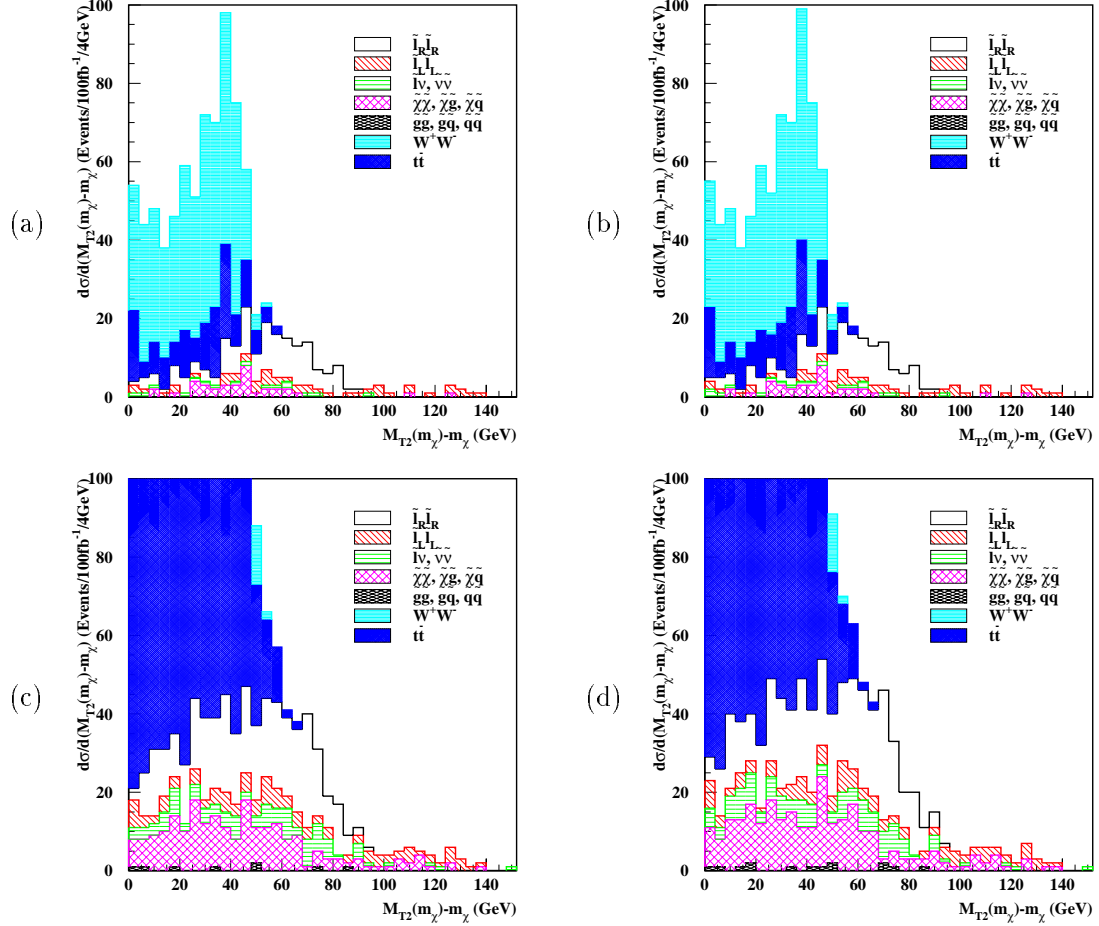
Figure 8: These M_{T2} distributions for O1 are generated from 100 events fb ^{-1} at high luminosity, and from the M_{T2} cuts described in section 3.4. (a) and (b) use the “hard” cuts, while (c) and (d) use the “soft” cuts. In (a) and (c), events containing a jet with p_T > 40 GeV were vetoed. In (b) and (d), this cut was relaxed to 50 GeV. In all plots, M_{T2}(\chi) is evaluated at \chi = m_{\tilde{\chi}_1^0} . The results are presented in the form M_{T2}(m_\chi) - m_\chi in order to show the edge of the signal region located at the difference between the slepton and neutralino masses (92.5 GeV).
