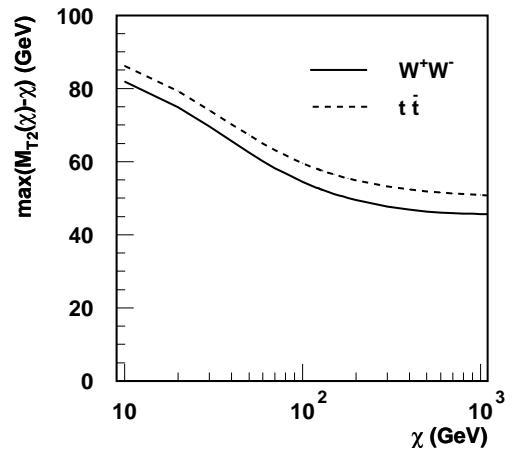
Figure 10: Variation with \chi of the SM contributions to \max(M_{T_2}(\chi) - \chi) (for a number of events corresponding to 100 \text{ fb}^{-1} ) which provides a measure of the minimum \tilde{l}-\tilde{\chi}_1^0 mass difference which is needed for signal M_{T_2} events to be able to extend beyond the SM backgrounds. Events contributing to this plot were selected using the “hard” M_{T_2} cuts.
