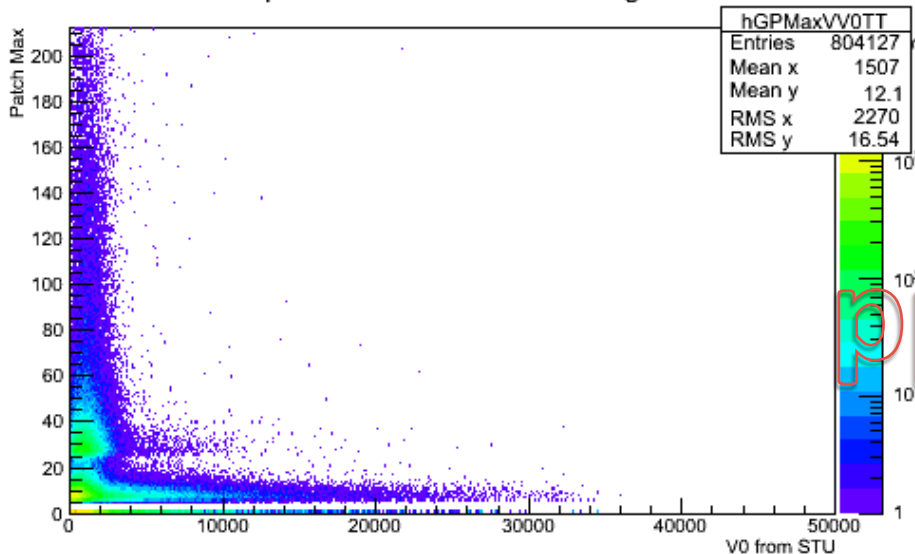
Maximum patch of L1-Gamma vs V0 signal in STU
