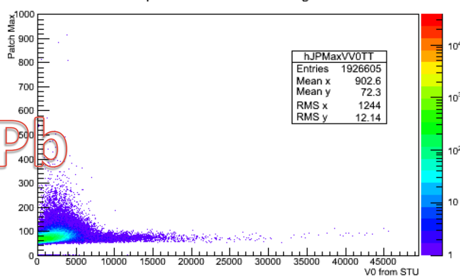
Maximum patch of L1-Jet vs V0 signal in STU
