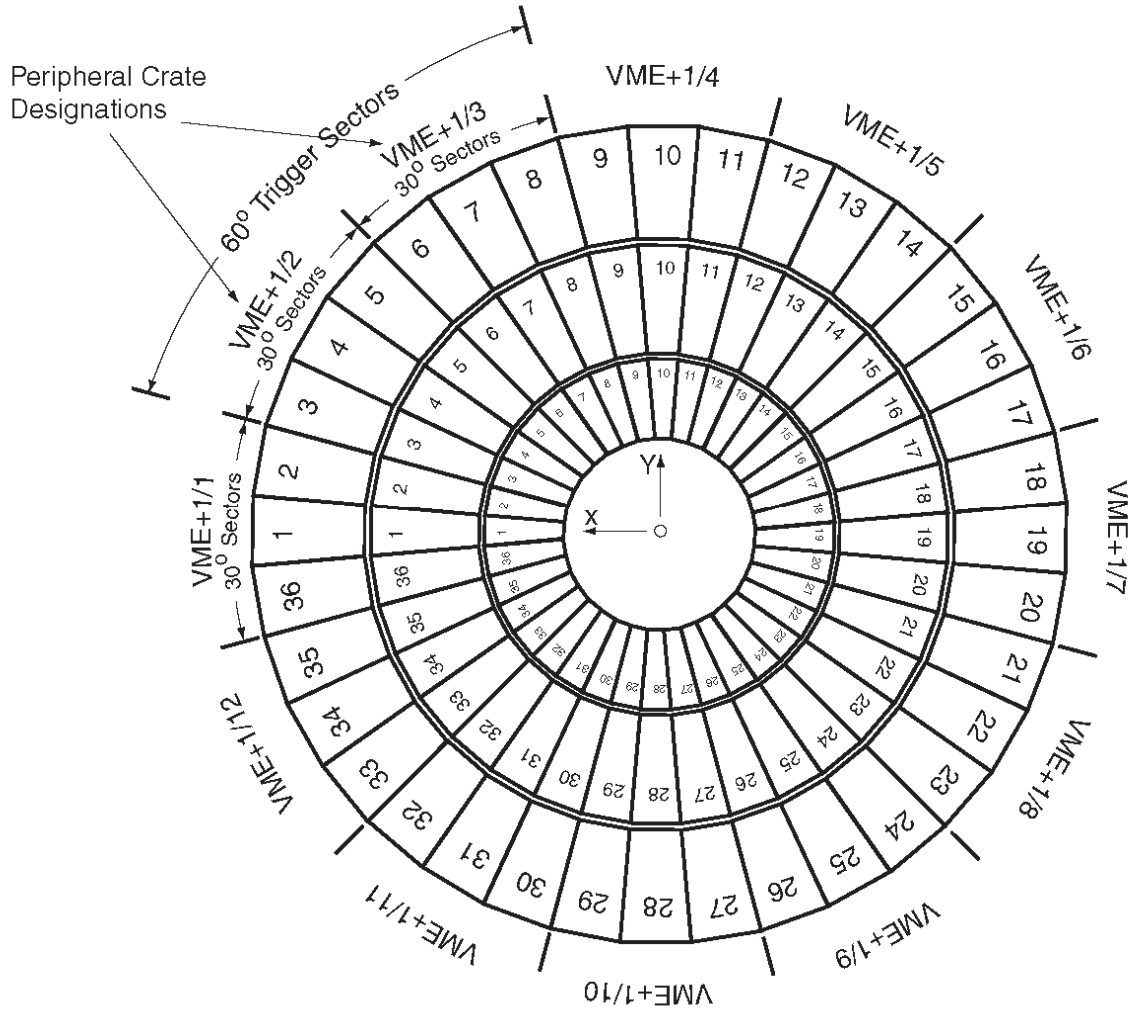
Figure 11. An r - \phi cross-section of the ME1 endcap muon station as viewed from z =negative infinity, showing the positions of chambers, trigger sectors, and correspondence to peripheral crate names. On the +z side, this is the same view as from the IP, while on the -z side, this is a view looking towards the IP.
