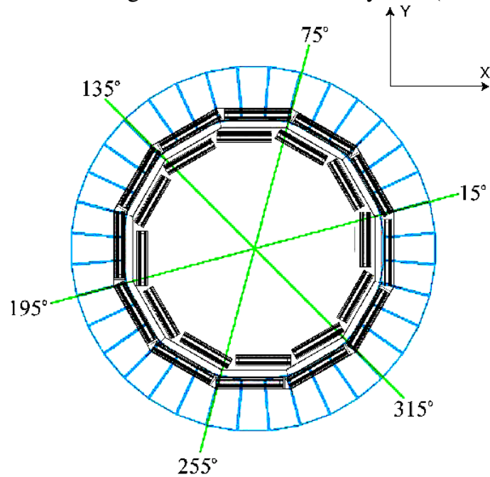
Figure 6. An r - \phi cross-section view of the barrel muon system, with the positions of the outer ring of endcap muon chambers superimposed (looking East, or towards the -z endcap). This diagram shows the edges of the 60° trigger sectors (ME2, ME3, and ME4) and the position of the outer (large) chambers.
