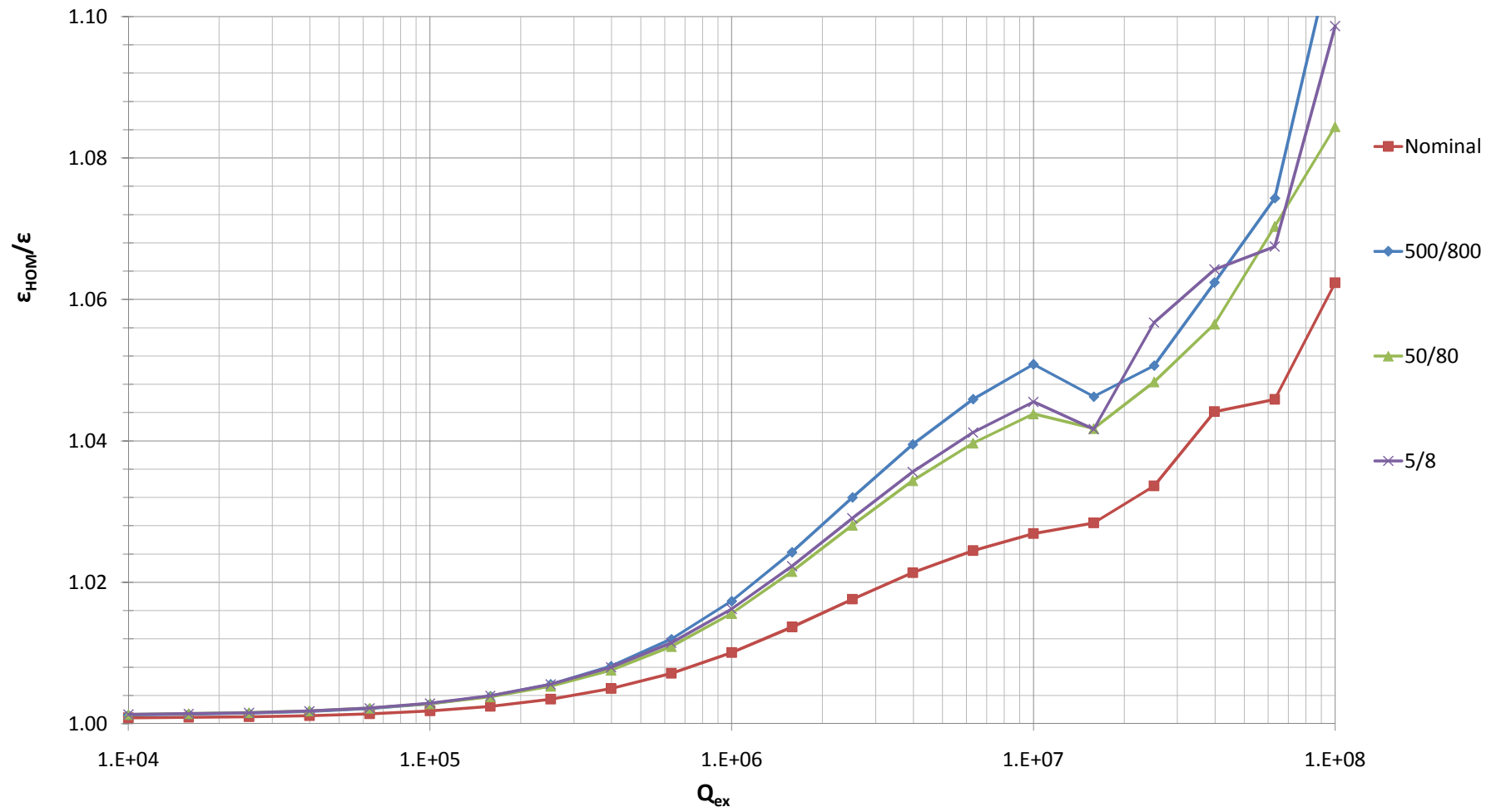
Emittance growth rate transversal WS parameter, R/Q(Beta), chopping, 400mA
