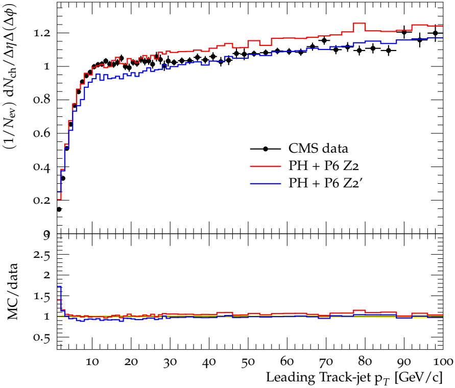
Profile N_{\text{ch}} at \sqrt{s} = 7 TeV, 60 < |\Delta\phi| < 120
