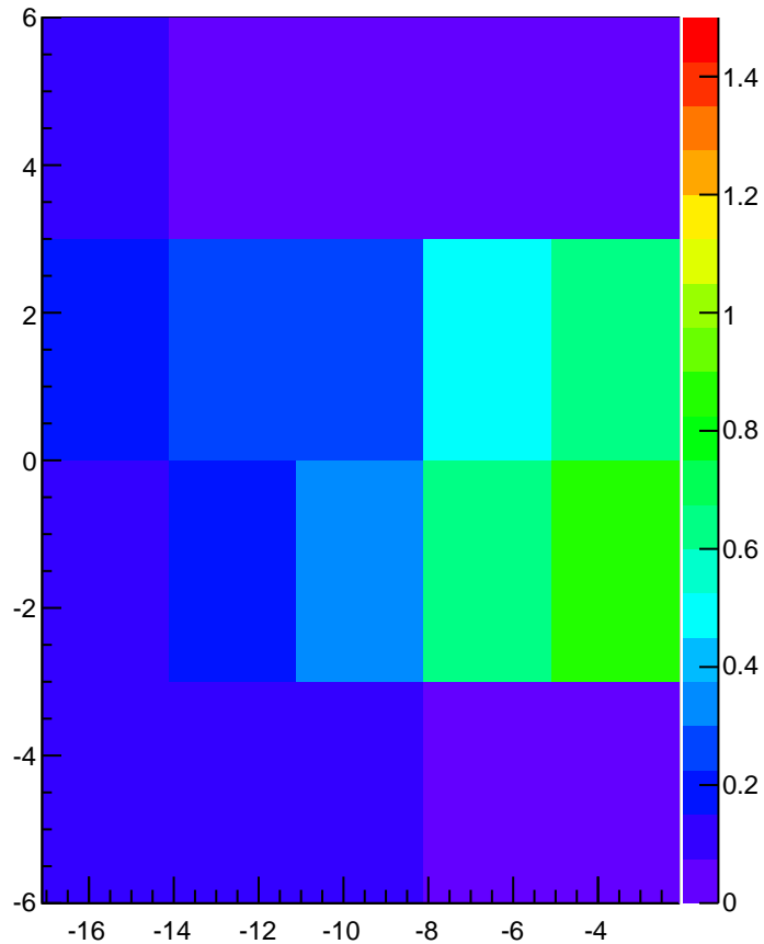
ToF Detector background occupancy, Signal+Pileup+Background
