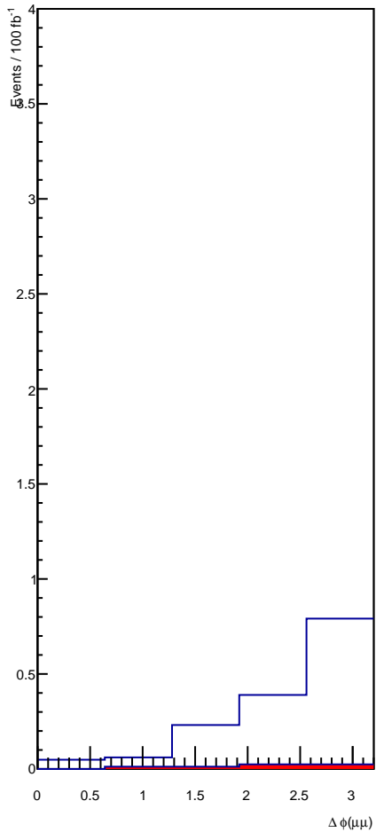
WW Signal MC, 10ps ToF, +-30ps vertex compatibility
